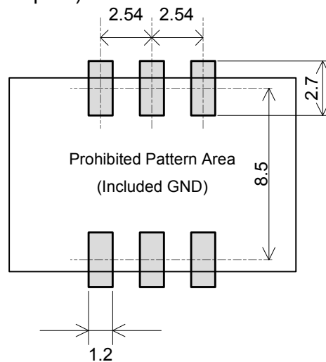
(Foot-print)
